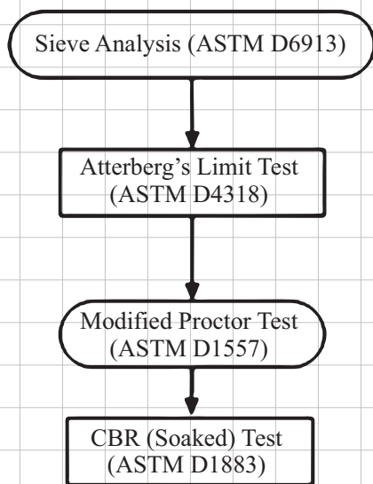
Fig. 2. Laboratory Testing Program [xix-xxii]
