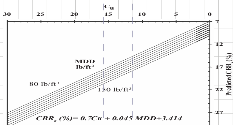
Fig. 13. Predictive Curve for Coarse grained soils (Eq. 10)
