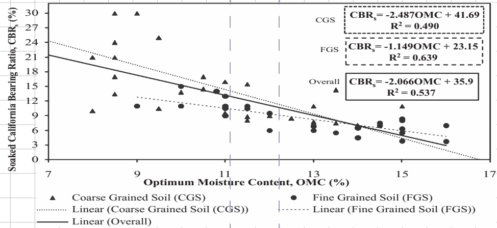
Fig. 4. Relationship between CBR soaked Value (%) and Optimum moisture content (%)
